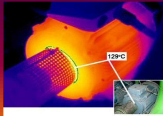
Overheating failure
