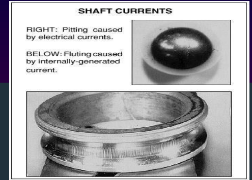
Bearing failure
